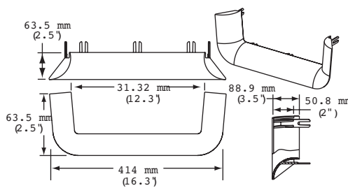
Trumpet Flare (FGS-MTRM-F)
