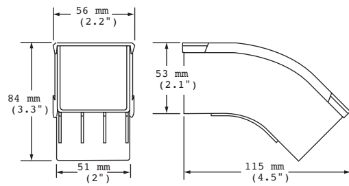
45° Down Elbow (FGS-MD4A-C)
