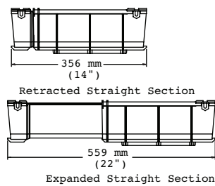
Expandable Straight Section (FGS-MVAR-A)
