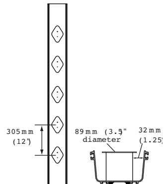
Slack Storage Straight Section (FGS-MSHS-STOR-B)
