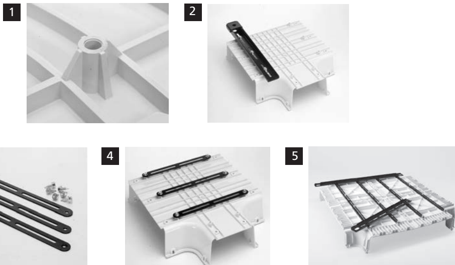
Variable Fitting Support Locator
