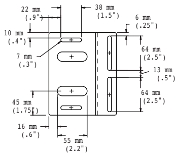
OMUX Frame Center Support Bracket Kit (FGS-HOMX-16MM)
