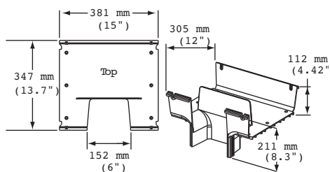
Downspout (FGS-MDSP-F)
