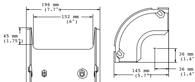
90° Down Elbow (FGS-MD9E-G)
