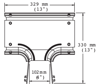
Extended Downspout (FGS-MDSP-EX-B)
