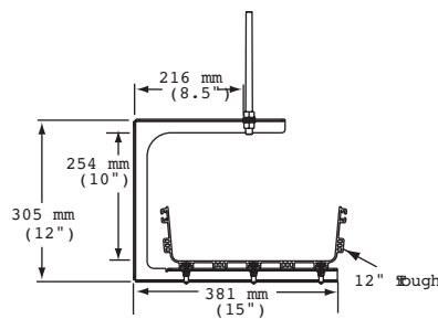
Top Support Threaded Rod C-Bracket Kit (FGS-HNTS-F-XX shown attached to 4x12 straight section)
