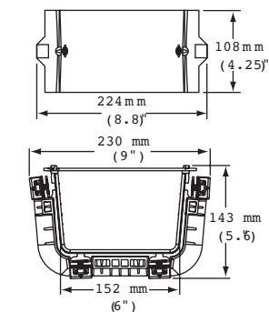
Snap-Fit Junction Assembly (FGS-MFAW-B)
