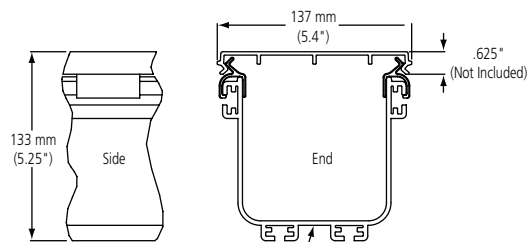
Snap-On Cover for 4\"/>
