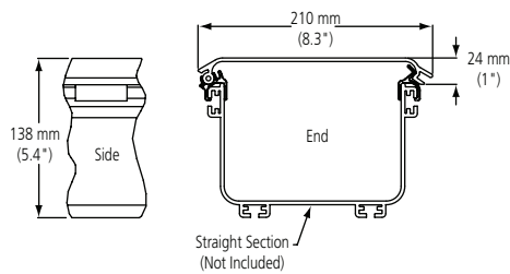
Hinged Cover for Straight Section (FGS-MSNC-B/G)
