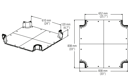
Horizontal Cross (FGS-MHXP-H)
